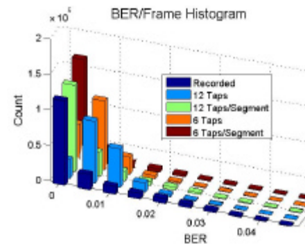
Figure 8: Histogram of the bit error rate for each processed frame
