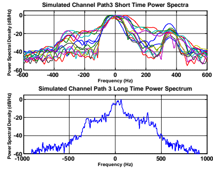
Figure 5: Simulated short time Doppler spectra and long time Doppler spectrum for the third tap of the 12 tap model scattering function
