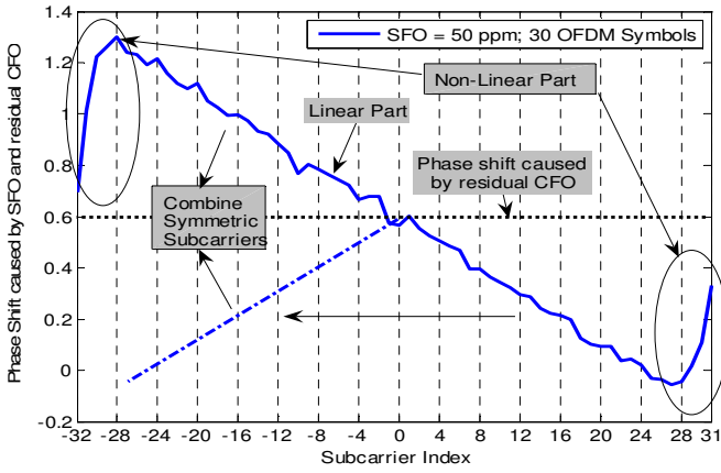
Fig. 1. Linearity and Symmetry of the Phase shift.
