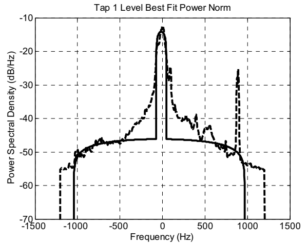
Figure 9: Two-shape fit to the random part spectrum of Tap No. 1.
