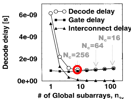
Figure 11a: Decode delay dependence on number of global subarrays, n_{1y} in Fig. 11 Figure 11b: Decode delay dependence on the number of subglobal subarrays n_{2x} in Fig. 11 Figure 11c (at right): Sense delay dependence on the number of subglobal subarrays n_{2x} in Fig. 10.
