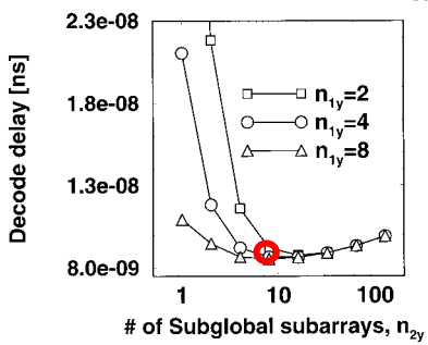
Figure 9a,b: Array architecture and decode network from [16]. Inverters following NAND gates not shown for simplicity. Figure 9c: Decode delay dependence on number of global ( n_{1y} ) and subglobal ( n_{2y} ) subarrays in Example 2. Dotted lines correspond to a constant total number of blocks.
