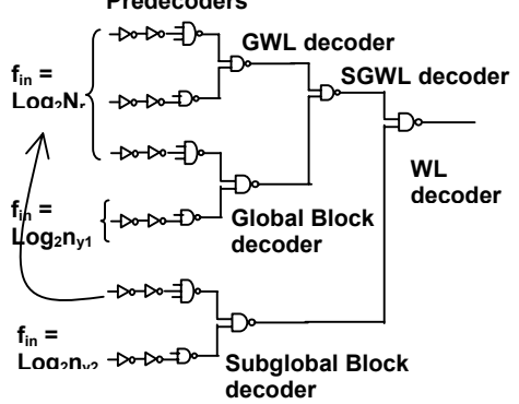
Figure 10b: Decode network of the SRAM array from [13] (Inverters following NAND gates are not shown for simplicity)
