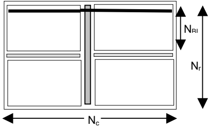
Figure 10a: Entire SRAM in [13] divided into array of 4 macros. Each macro divided into 8 global subarrays (not including redundancy) with global sense amplifiers placed above each global subarray. Each global subarray divided into n_2 subglobal subarrays. Each subglobal subarray has a height of N_r and width of N_c . The WL drivers are placed at the center of the subarray with N_{frac} = 2 . The BL is divided into two segments with d_{BL} = 2 with local sense amplifiers placed between these.
