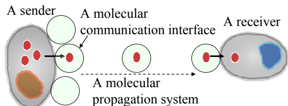
Figure 3. A molecular communication mechanism using vesicles.
