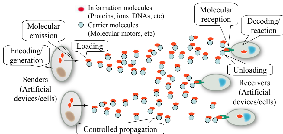
Figure 1. An example molecular communication system.
