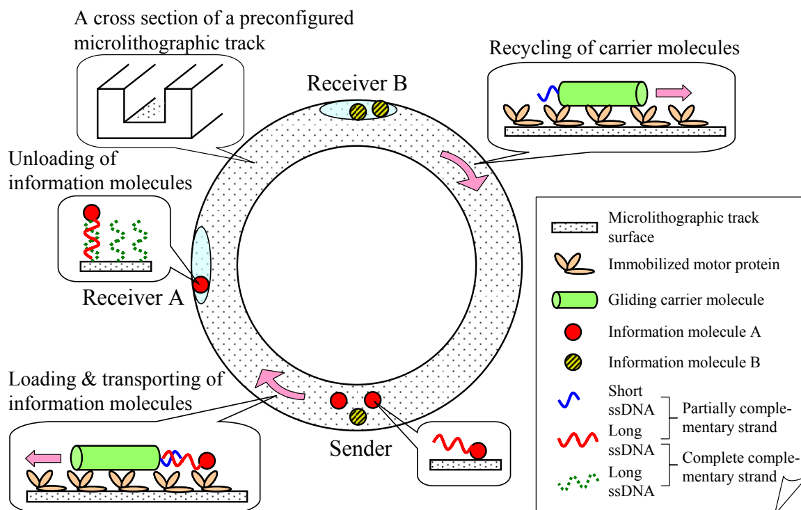
Figure 2. A schematic diagram of a molecular propagation system.
