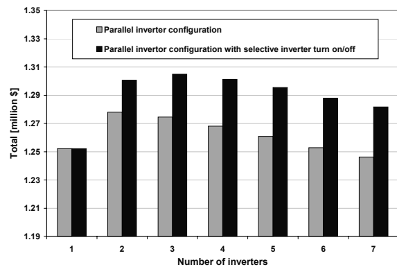
Fig. 5. The optimal number of inverters in the system.
