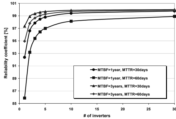
Fig. 4. The dependence of the reliability coefficient on the failure characteristics of the inverter and repair time.
