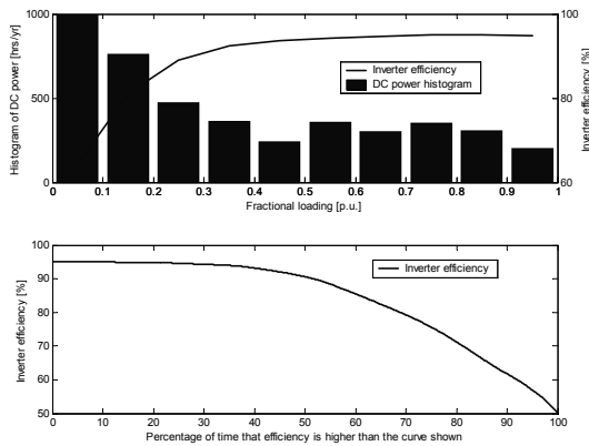
Fig. 1. (a) Typical PV inverter output histogram and its corresponding efficiency, (b) Efficiency duration curve.
