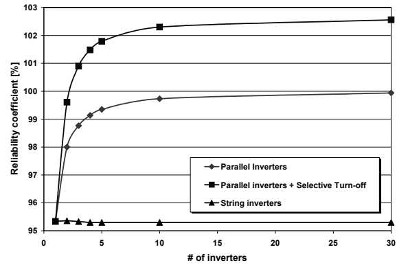
Fig. 3. The performance-adjusting reliability coefficient as a function of number of inverters in the system (using data from the GTAC PV system in Atlanta, GA).
